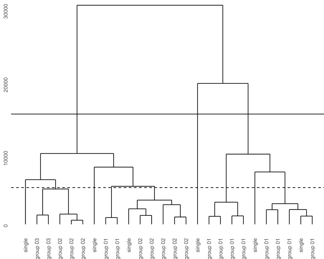
Figure 5.3. Cluster analysis and subsequent dendrogram of the dataset used in Fig. 5.2 and Fig. 5.1. Distances are calculated as euclidian distances, and clustering is done by the complete linkage method. Instead of sample names, group names are used to make comparison of the grouping methods more visible. The grouping done by NAA and statistical analysis (group01, group02 and group03) agrees with the archeological grouping of this dataset; the grouping that would follow from the dendrogram cannot be related to archeological groups.
